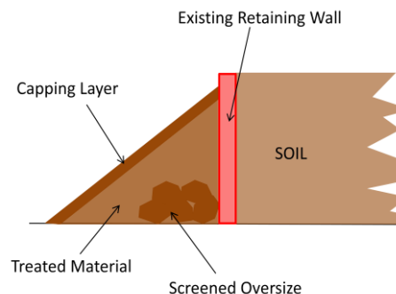
Figure 6 – Schematic Showing Reuse of Treated Material in a Batter
